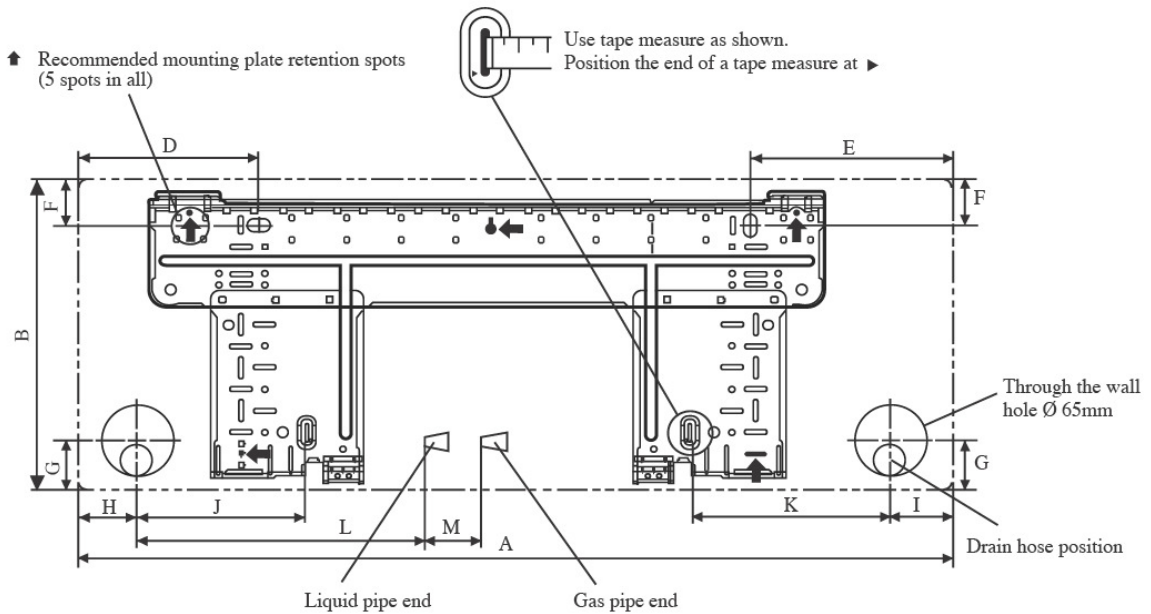
INSTALLATION PLATE 20/25/35
